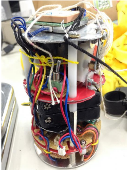
CanSat
